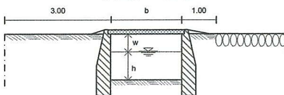
POTONGAN A - A H 1: 100 V 1: 100
