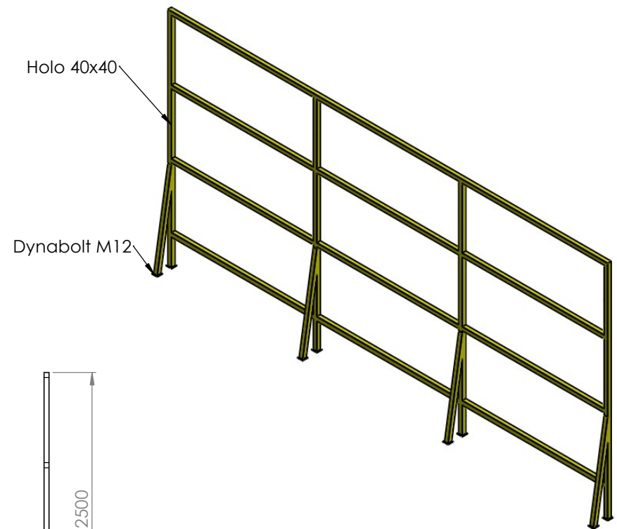
Isometric View
