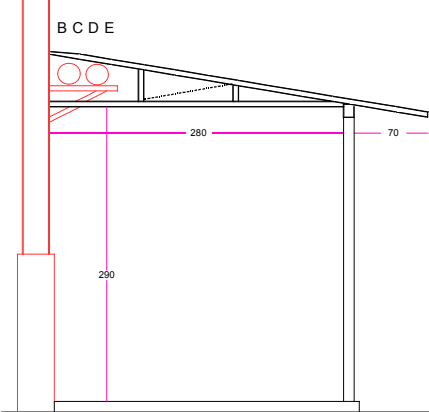
Roof Top Ruang Istirahat Lorong D 300X2400
