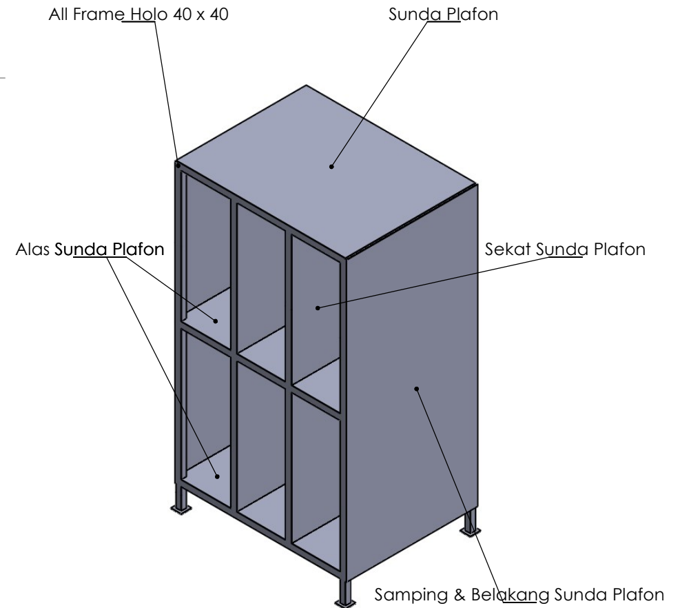
Isometric View
