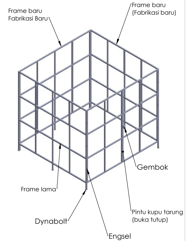
Isometric View
