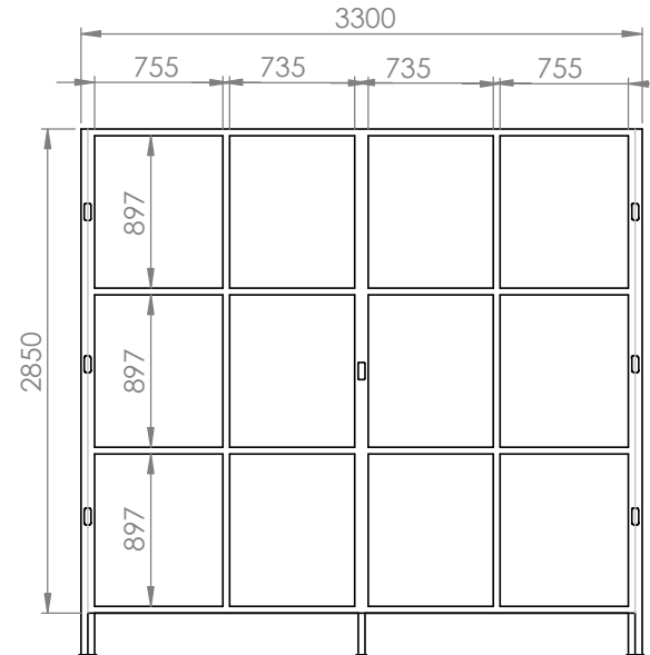
Side View Pintu
